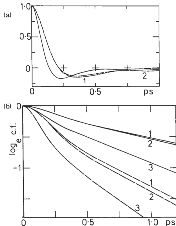
FIG. 2. (a) Dashed lines: (1), \langle \dot{\hat{e}}_1(t) \cdot \dot{\hat{e}}_1(0) \rangle / \langle \dot{\hat{e}}_1^2 \rangle , S enantiomer, laboratory frame; and (2), same as (1), R enantiomer. Solid line, same as for (1), racemic mixture. Note that the Fourier transforms of these functions give far-infrared spectra (Ref. 9). The far-infrared spectrum of the racemic mixture peaks at roughly twice the frequency of either enantiomer, whose spectra are identical within the computer-generated noise. (b) P_1 (first rank) (Refs. 8 and 9) and P_2 orientational ACF's of \hat{e}_1 , laboratory frame. Solid lines: (1), R enantiomer; (2), S enantiomer; (3) racemic mixture ( P_1 ). Dashed lines: (1), S enantiomer; (2), R enantiomer; (3), racemic mixture ( P_2 ). The P_1 functions can be related (Ref. 8) to infrared band shapes and dielectric loss curves, and the P_2 to Raman and Rayleigh spectra. The dielectric relaxation time from (b) is much shorter for the racemic mixture than for either enantiomer liquid.
