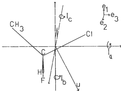
FIG. 1. The S enantiomer of 1,1-fluorochloroethane. The x , y , and z axes label the principal-moment-of-inertia frame, intersecting at the center of mass. The principal moments of inertia are I_a , I_b , and I_c . The direction of the resultant molecular dipole moment is labeled u . Inset: The frame of the unit vectors \hat{e}_1 , \hat{e}_2 , and \hat{e}_3 (see text). The R enantiomer is obtained by holding a mirror to the plane of the paper, i.e., by interchanging the positions of H and F.
